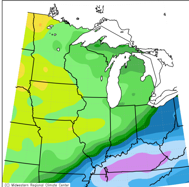
Accumulated Precipitation (in) February 1, 2025 to February 28, 2025
