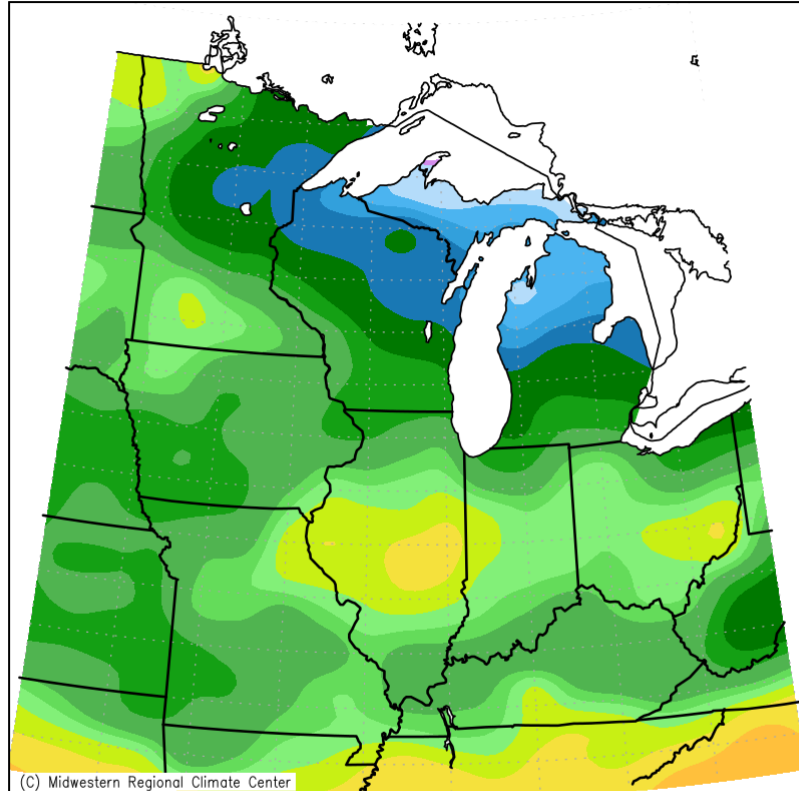
Accumulated Snowfall (in) February 1, 2025 to February 28, 2025
