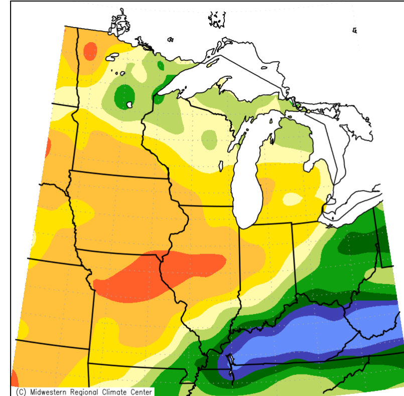
Accumulated Precipitation: Percent of Mean February 1, 2025 to February 28, 2025
