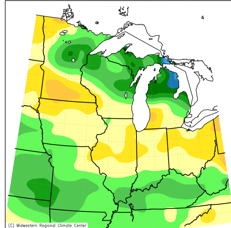
Accumulated Snowfall (in): Departure from Mean February 1, 2025 to February 28, 2025
