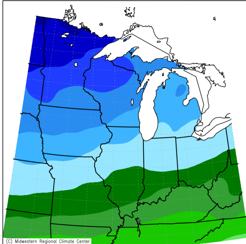
Average Temperature (°F) February 1, 2025 to February 28, 2025
